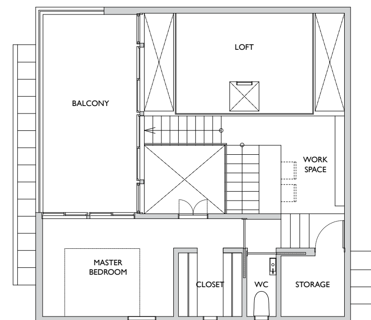
Loft level plan
